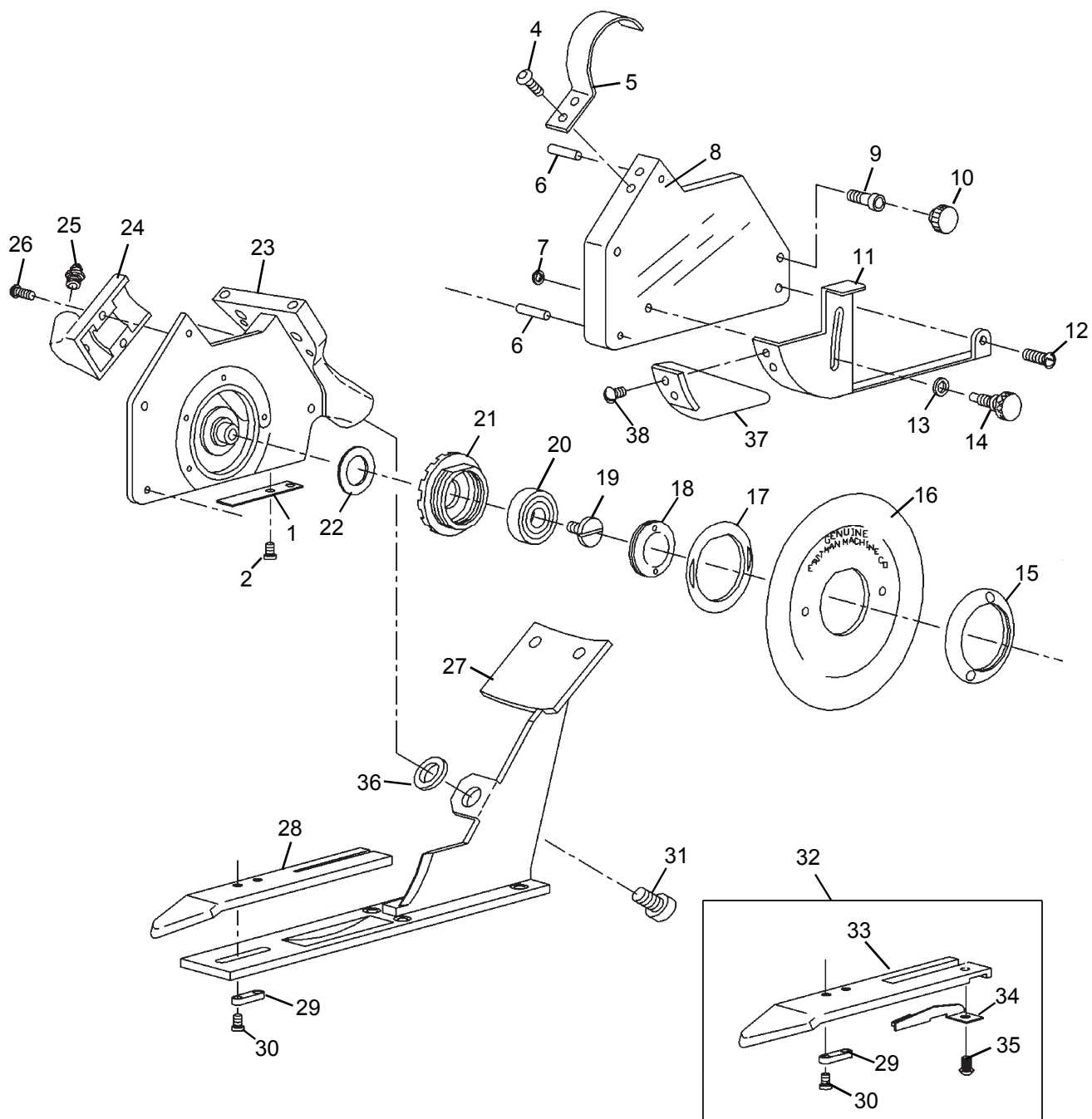
SHEAR THROAT PLATE ASSEMBLY
